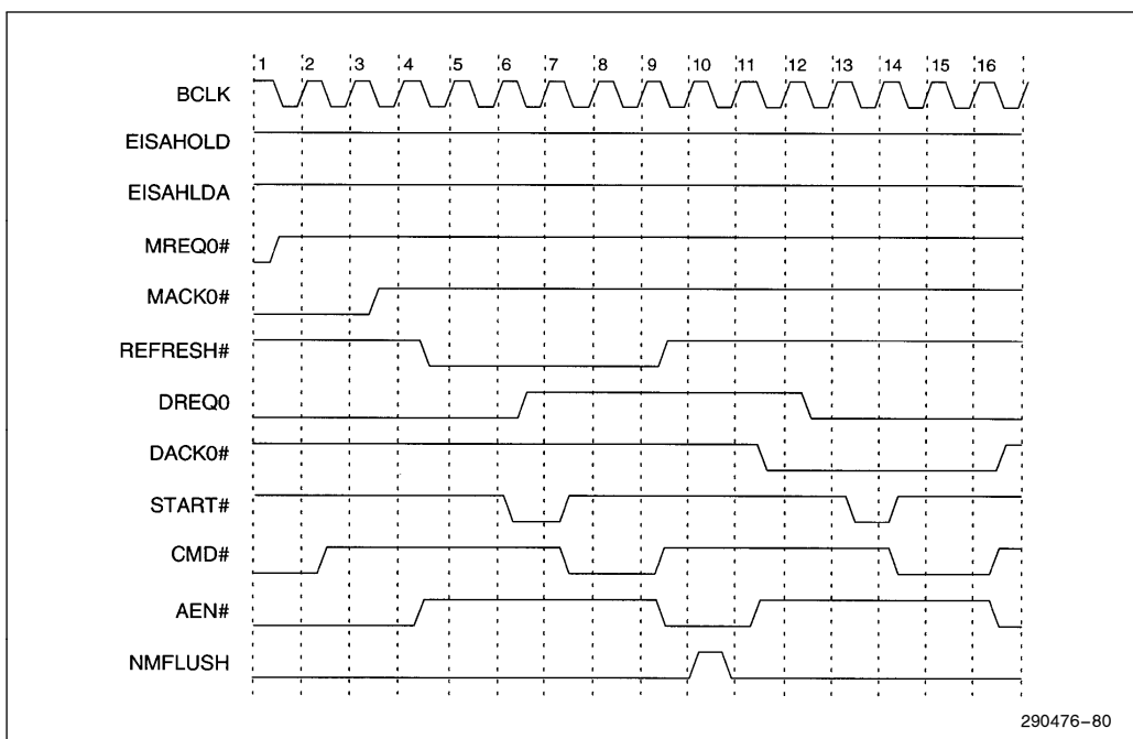
Figure 17. EISA Arbitration
